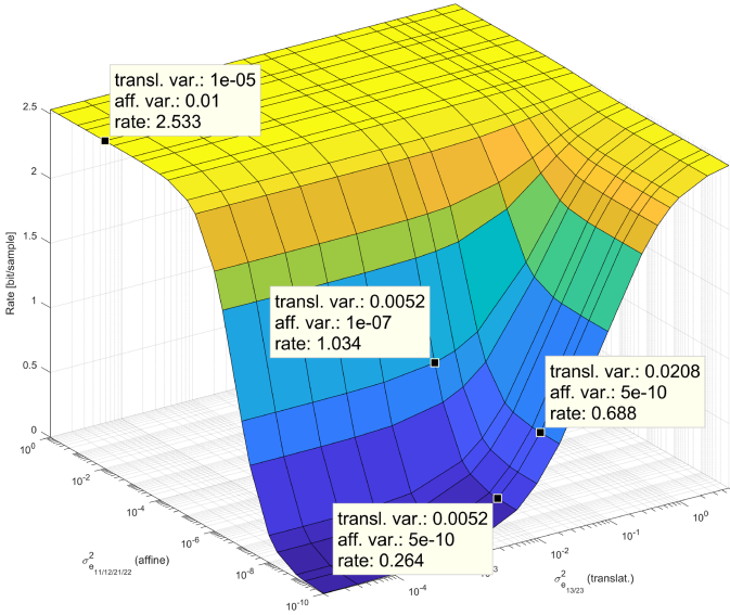
Fig. 3. Minimum required bit rate versus variances \sigma_{e_{ij}}^2 for a distortion of SNR = 30 dB assuming \sigma_{e_{11}}^2 = \sigma_{e_{12}}^2 = \sigma_{e_{21}}^2 = \sigma_{e_{22}}^2 (called \sigma_{e_{\text{aff.}}}^2 in (b)) and \sigma_{e_{13}}^2 = \sigma_{e_{23}}^2 for HD resolution.
