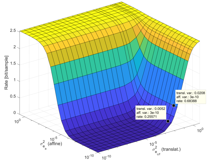
Fig. 4. Minimum required bit rate versus variances \sigma_{e_i}^2, i = a, b, c, f of Gaussian displacement estimation error pdfs for SNR = 30 dB assuming \sigma_{e_b}^2 = 2\sigma_{e_a}^2 and \sigma_{e_c}^2 = \sigma_{e_f}^2 (block size 64 \times 64 pel, transform center in the middle of the block) [30].
