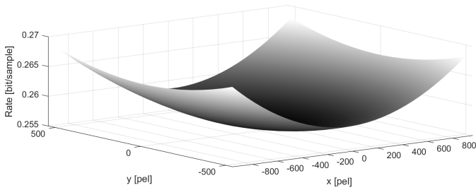
Fig. 2. Location-dependent bit rate for a HD frame and maximum accurate non-translational affine estimation ( \sigma_{e_{11}}^2 = \sigma_{e_{12}}^2 = \sigma_{e_{21}}^2 = \sigma_{e_{22}}^2 = 5 \cdot 10^{-10} ) and translational quarter-pel resolution.
