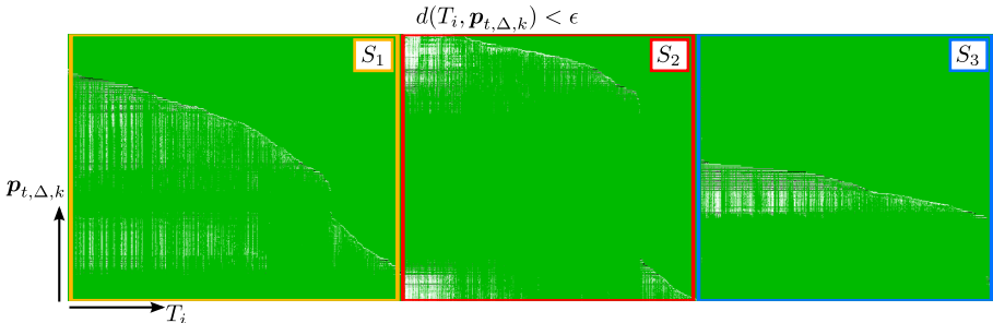
Fig. 4. Preferred motion parameters \mathbf{p}_{t, \Delta, k} of 6795 trajectories and 768 frame-to-frame motions from the bookstack sequence (Section 4.3). Several objects are occluded at the same time. White denotes inliers, black outliers and green missing data (98.5%), e.g. due to occlusion. \mathcal{S}_2 corresponds to the lowest book and \mathcal{S}_3 to the topmost (cf. Fig. 8).
