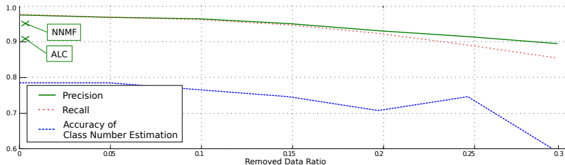
Fig. 6. Average precision, recall and class number estimation accuracy from Section 4.2 over the ratio of removed data. The precisions from ALC and NNMF are extracted from [7].
