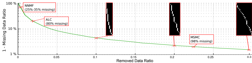
Fig. 5. Simulation how removed data affects missing data. The three binary images are examples of the result of one trajectory getting split because of gaps from 10%, 20%, and 30% removed data. The images show if data is known (white) or missing (black) for different resulting trajectories (columns) over time (rows).
