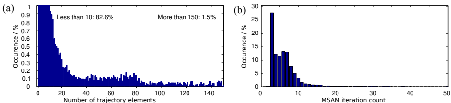
Fig. 7. (a) Histogram of the number of known trajectory elements for the bookstack sequence (Section 4.3). (b) Histogram of MSAM iteration count of all frames, scales and sequences of the experiment in Section 4.1.
