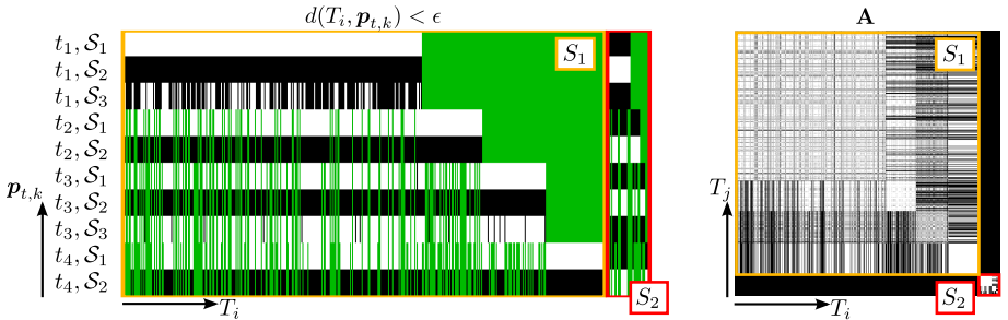
Fig. 3. Left: Preferred motion parameters \mathbf{p}_{t,k} of trajectory T_i , clustered by motions S_1 (yellow) and S_2 (red). White denotes inliers, black outliers and green missing data (no observation of T_i at frame t ). Right: Corresponding affinity matrix \mathbf{A} of the affinity between trajectories T_i and T_j .
