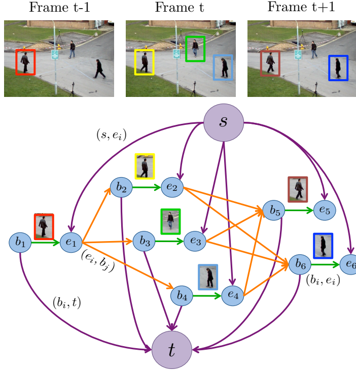
Fig. 2: Example of a graph with the special source s and sink t nodes, 6 detections which are represented by two nodes each: the beginning b_i and the end e_i .
