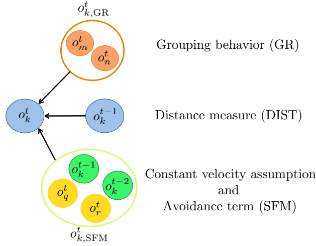
Fig. 5: Diagram of the dependencies for each observation \mathbf{o}_k^t .
