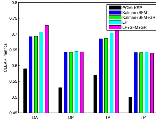
Fig. 12: Results of the proposed method on the PETS2009 dataset views 1. (a) Detection accuracy, DA. (b) Detection precision, DP. (c) Tracking accuracy, TA. (d) Tracking precision.
