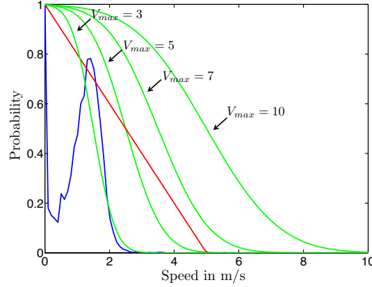
Fig. 3: Blue = normalized histogram of speeds learned from training data. Red = probability distribution if cost depends linearly on the velocity. Green = probability distribution if the relation of cost and velocities is expressed by Equation (13). An V_{\max} = 7m/s is used in the experiments.
