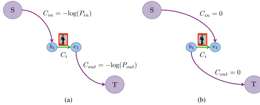
Fig. 4: (a) Graph structure as used in [40], which requires the computation of P_{in} and P_{out} in an Expectation-Maximization step during optimization. (b) Graph structure as used in [21] which does not require the computation of these two parameters; the trajectories are found only with the information of the link and detection edges.
